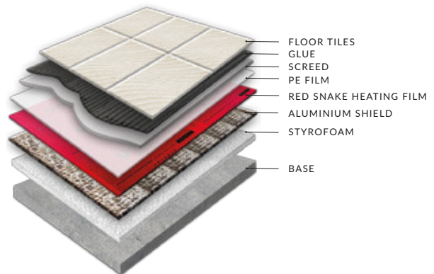
INSTALLATION ARRANGEMENT FOR TILED FLOORS
