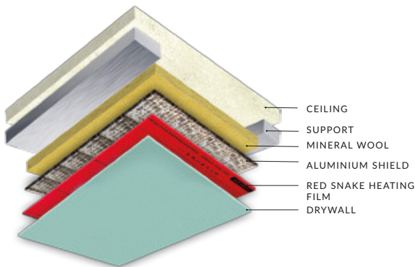
INSTALLATION ARRANGEMENT FOR CEILINGS
